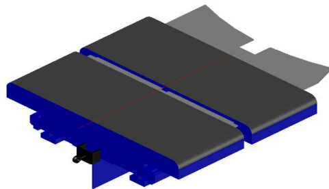
CBS Carrier
