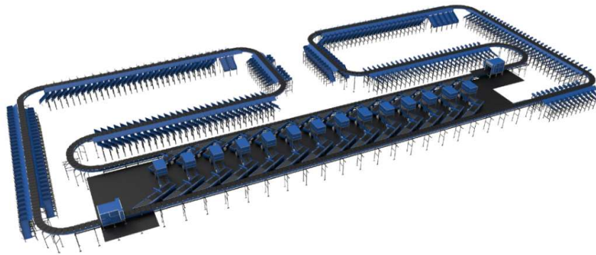
Cross Belt Sorter
